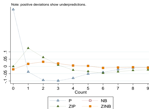
Figure 5: Comparisons among observed versus predicted probabilities among count models for methadone
