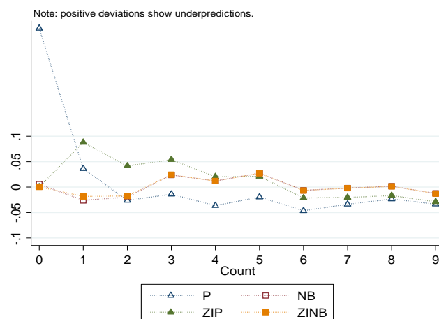
Figure 4: Comparisons among observed versus predicted probabilities among count models for alcohol
