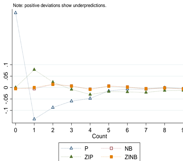
Figure 6: Comparisons among observed versus predicted probabilities among count models for female sex worker
