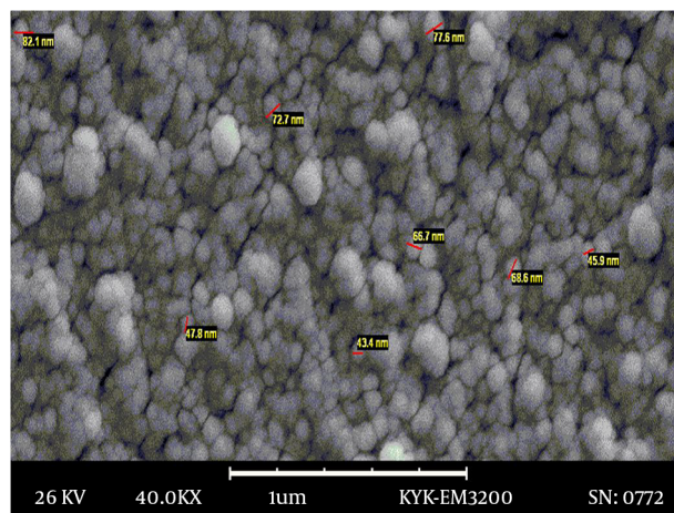
Figure 4. Image of nanoparticles with greater magnification
