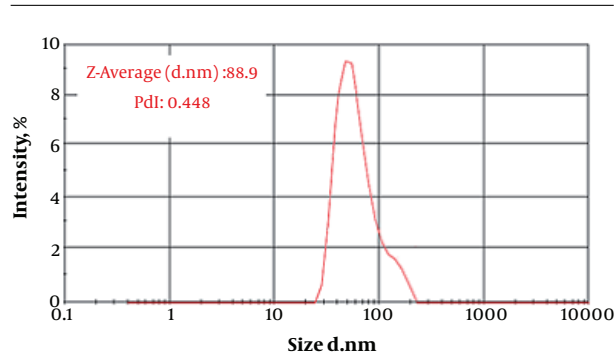
Figure 1. Curve of Particle Size Distribution of Fluconazole-loaded Liposomes
