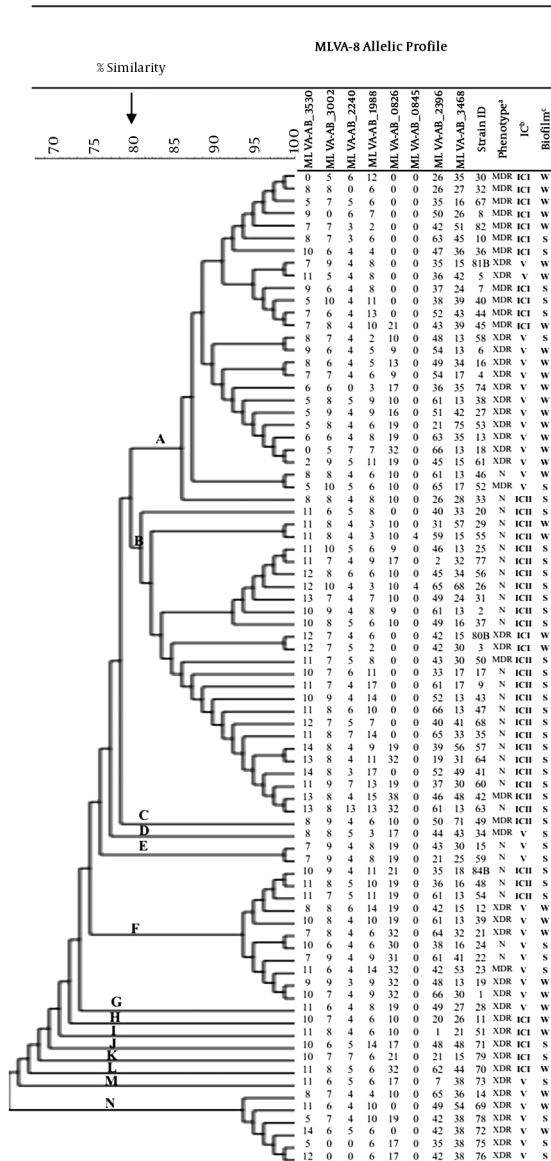
Figure 2. Dendrogram of genetic diversity of A. baumannii isolated from burn patients by MLVA, biofilm formation, international clone, and resistant phenotypes. Abbreviations: MDR, multidrug-resistant; XDR, extensively drug-resistant; N, non-MDR; IC, international clone; Biofilm formation: S, strong; W, weak.
