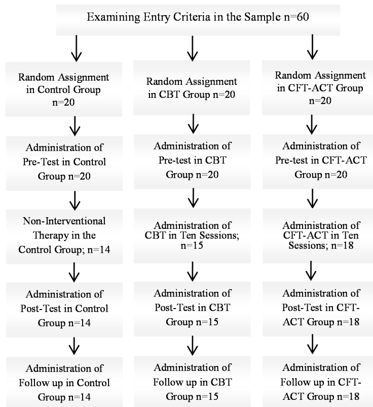
Figure 1. Consort flowchart
