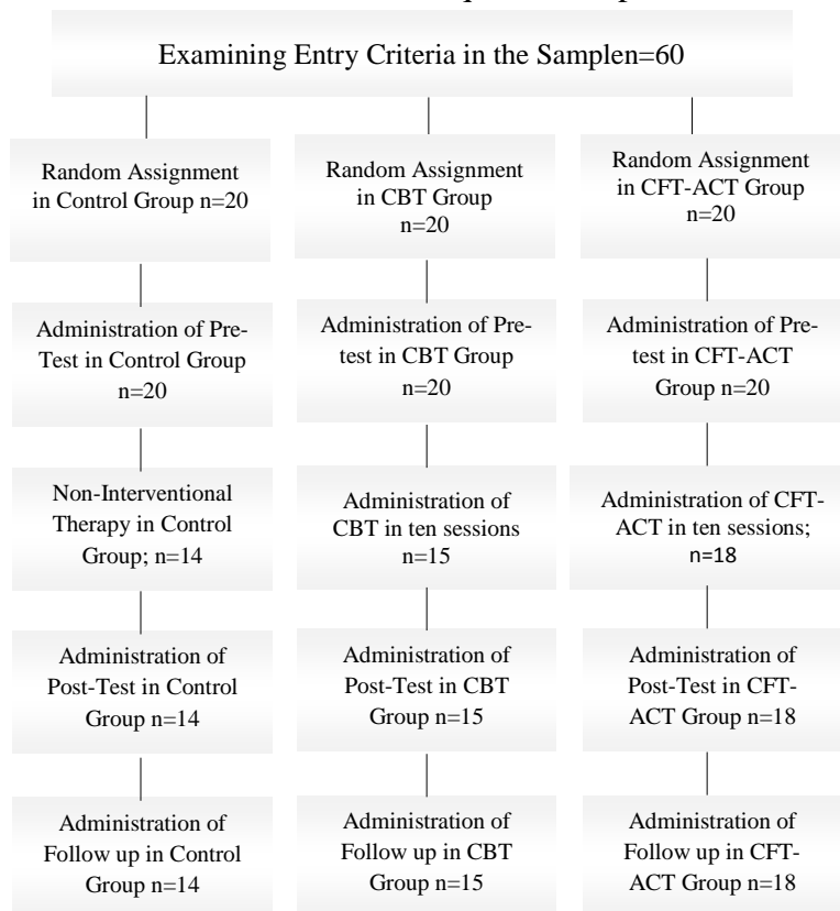
Figure 1. Consort Flowchart
