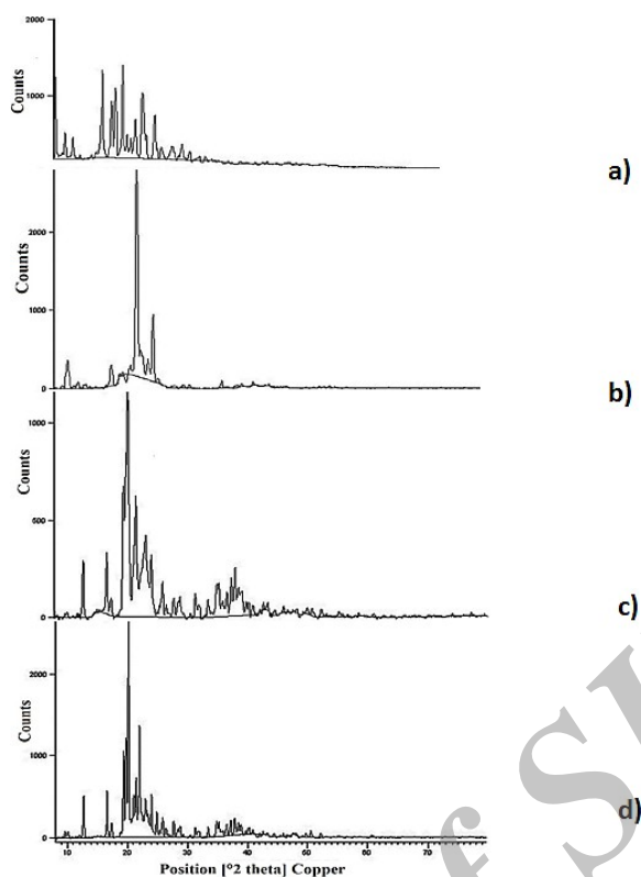
Fig. 5. a) XRD of candesartan cilexetil, b) XRD of binary system with lipophilic excipient, c) XRD of physical mixture of formulation F3, d). XRD of formulation F3
