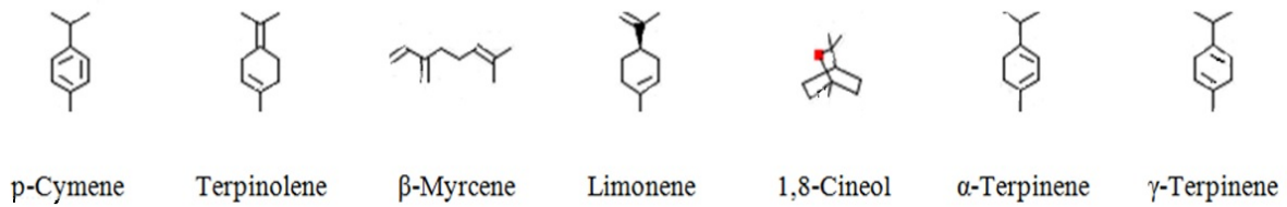
Fig. 5. Chemical structures of the main compounds of the toluene- ethyl acetate fraction.
