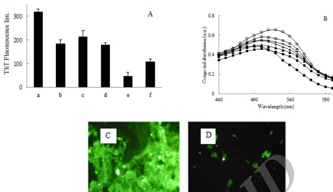
Fig. 1. Effect of the different organic fractions of Cuminum cyminum oil on the aggregation of hen egg white lysozyme. Fibrillation was estimated by A; thioflavin T fluorescence intensity and B; congo red absorbance in the absence (a,○) and presence of the fractions, b; n-hexane (□), c; n-hexane/toluene (-), d; toluene (Δ), e; toluene/ethyl acetate (■), f; ethyl acetate (▲) and congo red (●). The samples were incubated at 57 °C/24 h. Fluorescence microscopic images of C; hen egg white lysozyme incubated for 48 h in the absence and D; the presence of the toluene-ethyl acetate fraction. The stated errors are the SDs of three repeated experiments.
