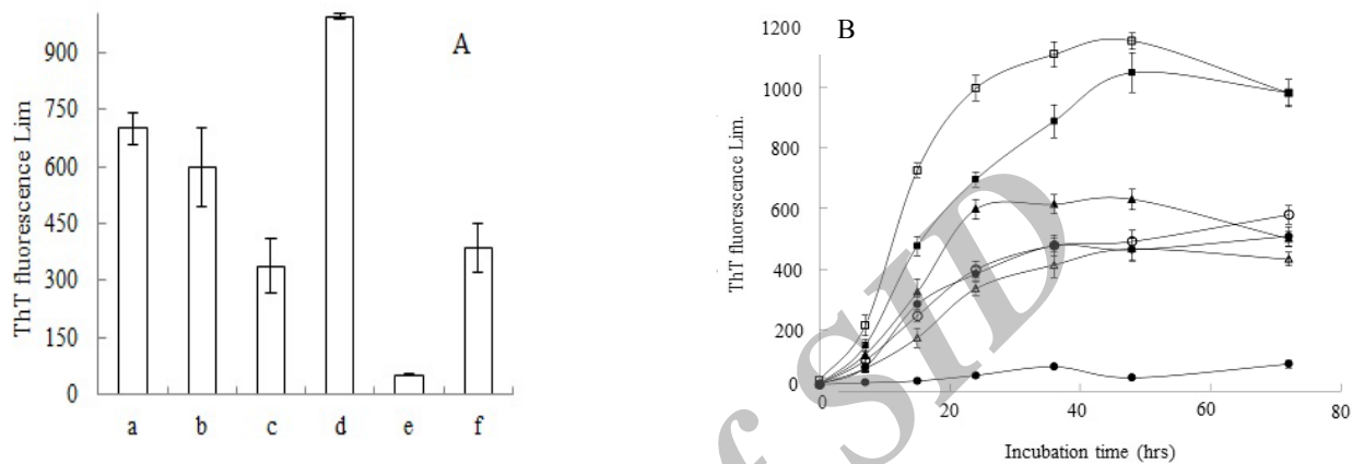
Fig.6. The effects of the test samples on the aggregation of hen egg white lysozyme . Fibril formation of hen egg white lysozyme fibrillation was estimated by A; Thioflavin T fluorescence emission, and also B; kinetics of fibrillation in the absence (a,○) and presence of small molecules including b: 1,8 cineol (▲), c: p-cymene (Δ), d: limonene (□), e: terpinolene (●), f: \beta -myrcene (■). The samples were incubated at 57 °C. The stated errors are the SDs of three repeats. The results were significantly different from those of the a; control except 1,8 cineol ( P < 0.05 ).
