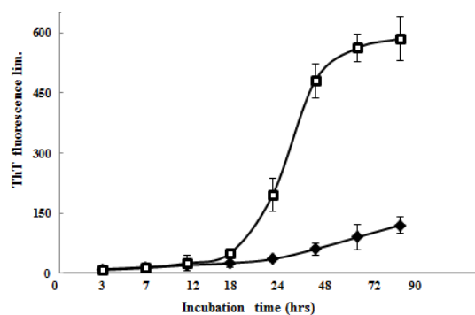
Fig. 2. The effect of the toluene-ethyl acetate fraction (5% (v/v)) on the kinetics of the fibrillation process. Time-study of the ThT fluorescence at 481 nm during
