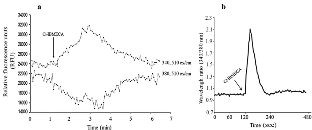
Fig. 3. A3AR mediated elevation of intracellular Ca^{2+} in MIN6 cells. Fura 2/AM (5 \mu M) was loaded to cells for 1 h and then these cells were stimulated with Cl-IBMECA (1 \mu M) for 8 min. (a) Fura 2 was stimulated at 340/510 and 380/510 nm to distinguish between Ca^{2+} bound and free forms of Fura 2, respectively. (b) 340/380 Ratio has been evaluated to indicate elevation of intracellular Ca^{2+} following Cl-IBMECA treatment. These assays were triplicated in three independent evaluations ( n = 9 ) and results presented as mean \pm SD. A3AR, Adenosine receptor; Cl-IBMECA, A3AR agonist.
