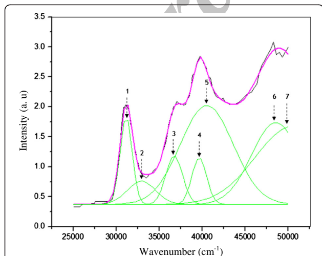
Figure 4 Deconvolution of the absorption spectrum of YAB-doped \text{Ce}^{3+} measured at 300 K. The green curves correspond to the deconvoluted absorption bands. The pink curve represents the absorption spectrum obtained by the deconvolution.
