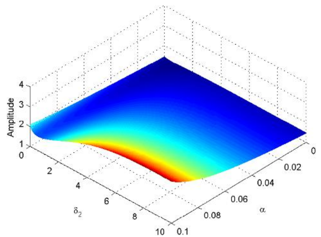
Fig. 6 The variation of the amplitude of the positive MZK solitary potential ( \phi_m^{(0)} > 0 ) with \delta_2 and \alpha for u_0 = 1, \delta_1 = 0.4, \beta_1 = 0.1, \beta_2 = 0.4 , and \theta = 30^\circ
