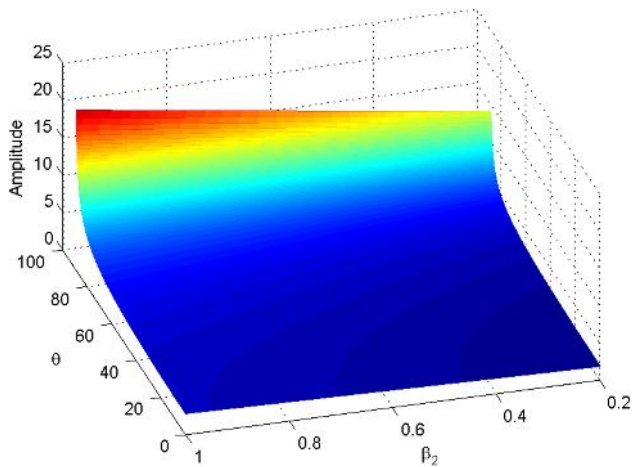
Fig. 7 The variation of the amplitude of the positive MZK solitary potential ( \phi_m^{(0)} > 0 ) with \beta_2 and \theta for u_0 = 1, \delta_1 = 1.1, \beta_1 = 0.1, \delta_2 = 2.1, and \alpha = 0.1
