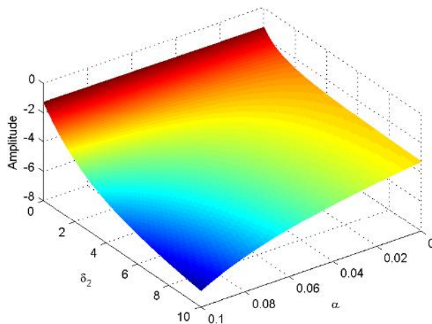
Fig. 2 The variation of the amplitude of the negative ZK solitary potential ( \phi_m^{(0)} < 0 ) with \delta_2 and \alpha for u_0 = 1 , \delta_1 = 0.1 , \beta_1 = 0.1 , \beta_2 = 0.4 , and \theta = 30^\circ
