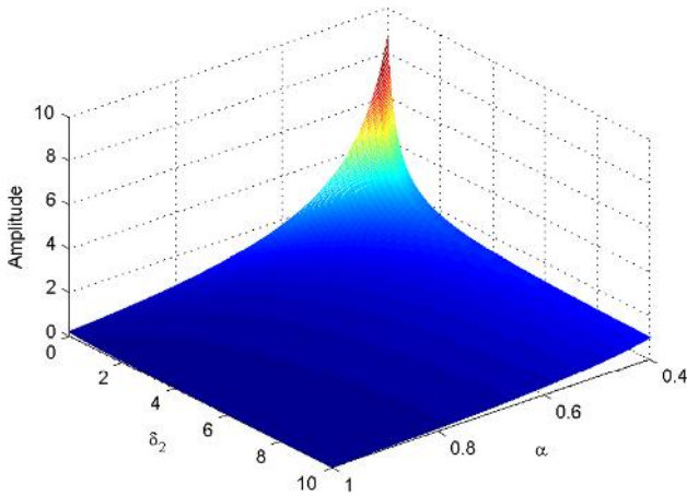
Fig. 3 The variation of the amplitude of the positive ZK solitary potential ( \phi_m^{(0)} > 0 ) with \delta_2 and \alpha for u_0 = 1, \delta_1 = 1.9, \beta_1 = 0.1, \beta_2 = 0.4 , and \theta = 30^\circ
