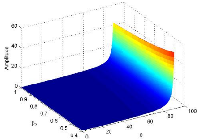
Fig. 5 The variation of the amplitude of the positive ZK solitary potential ( \phi_m^{(0)} > 0 ) with \beta_2 and \theta for u_0 = 1, \delta_1 = 1.2, \delta_2 = 2.1, \beta_1 = 0.1 , and \alpha = 0.5
