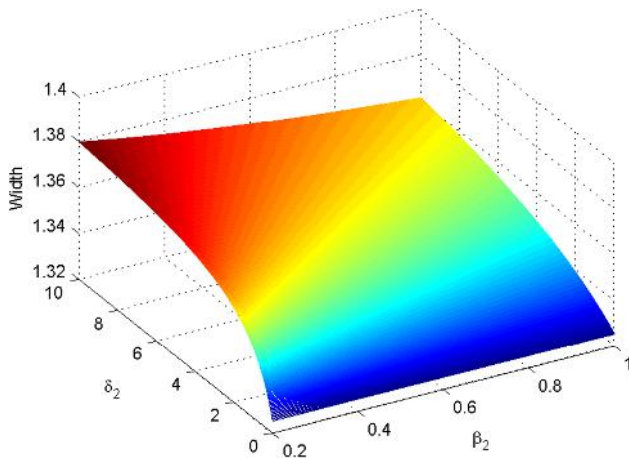
Fig. 11 The variation of the width of negative MZK solitary potential ( \phi_m^{(0)} < 0 ) with \delta_2 and \beta_2 for u_0 = 1, \delta_1 = 0.6, \beta_1 = 0.1, \alpha = 0.1, \theta = 30^\circ , and \omega_{cd} = 0.4
