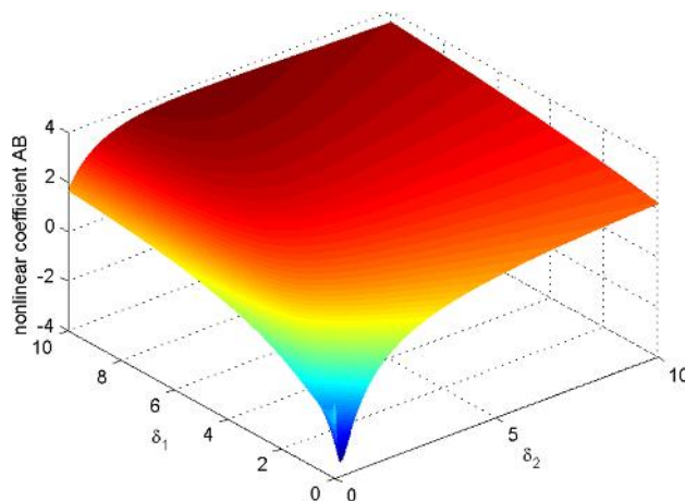
Fig. 1 The variation of the nonlinear coefficient AB with \delta_1 and \delta_2 for u_0 = 1 , \alpha = 0.4 , \beta_1 = 0.1 and \beta_2 = 0.4
