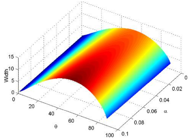
Fig. 10 The variation of the width of negative MZK solitary potential ( \phi_m^{(0)} < 0 ) with \theta and \alpha for u_0 = 1, \delta_1 = 0.6, \delta_2 = 2.1, \beta_1 = 0.1, \beta_2 = 0.4, and \omega_{cd} = 0.6
