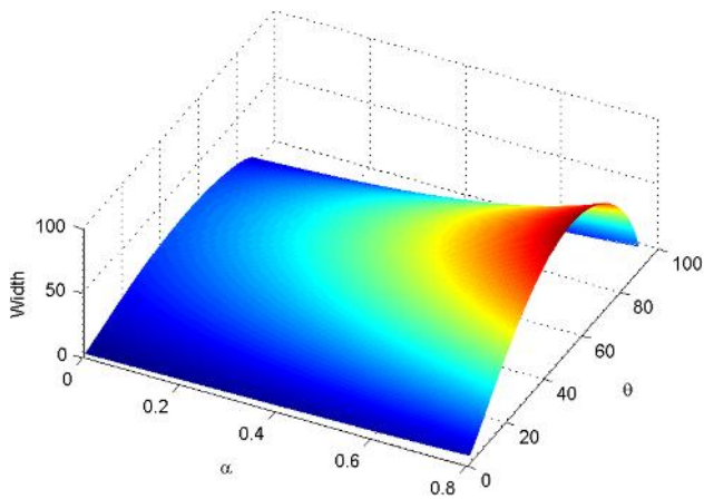
Fig. 8 The variation of the width of positive ZK solitary potential ( \phi_m^{(0)} > 0 ) with \theta and \alpha for u_0 = 1, \delta_1 = 0.6, \delta_2 = 2.1, \beta_1 = 0.1, \beta_2 = 0.4, and \omega_{cd} = 0.6
