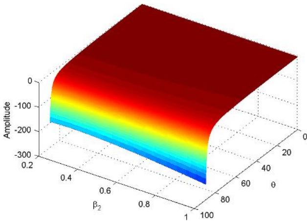
Fig. 4 The variation of the amplitude of the negative ZK solitary potential ( \phi_m^{(0)} < 0 ) with \beta_2 and \theta for u_0 = 1, \delta_1 = 0.1, \delta_2 = 2.1, \beta_1 = 0.1 , and \alpha = 0.1
