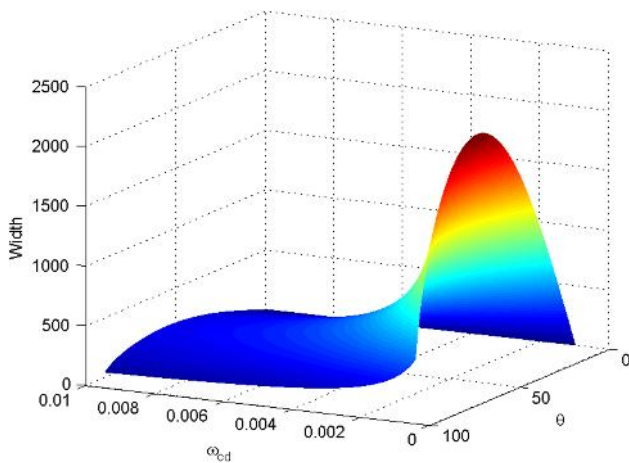
Fig. 12 The variation of the width of positive ZK solitary potential ( \phi_m^{(0)} > 0 ) with \omega_{cd} and \theta for u_0 = 1, \delta_1 = 0.1, \delta_2 = 2.1, \beta_1 = 0.1, \beta_2 = 0.4 , and \alpha = 0.5
