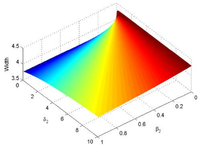
Fig. 9 The variation of the width of positive ZK solitary potential ( \phi_m^{(0)} > 0 ) with \delta_2 and \beta_2 for u_0 = 1, \delta_1 = 0.4, \beta_1 = 0.1, \alpha = 0.2, \theta = 30^\circ, and \omega_{cd} = 0.3
