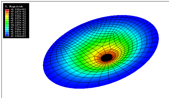
Fig. 2 First deformed mode shape and frequency parameter of a circular plate with clamped outer boundary (E = 200 \text{ GPa}, \rho = 7800 \text{ kg/m}^3, a = 1 \text{ m}, a_1 = 0.1 \text{ m} e = 0.1 \text{ m}, h = 0.02 \text{ m}, (r'_1, \theta_1) = (0.2 \text{ m}, 0^\circ), M = 100 \text{ kg}) .
