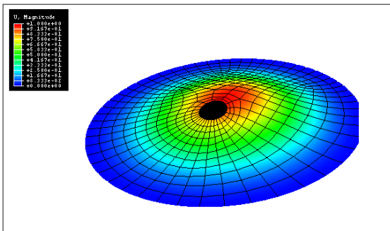
Fig. 4 First deformed mode shape and frequency parameter of a circular plate with clamped outer boundary (E = 200 \text{ GPa}, \rho = 7800 \text{ kg/m}^3, a = 1 \text{ m}, a_1 = 0.1 \text{ m} e = 0.1 \text{ m}, h = 0.02 \text{ m}, (r'_1, \theta_1) = (0.2 \text{ m}, 180^\circ), M = 100 \text{ kg}) .
