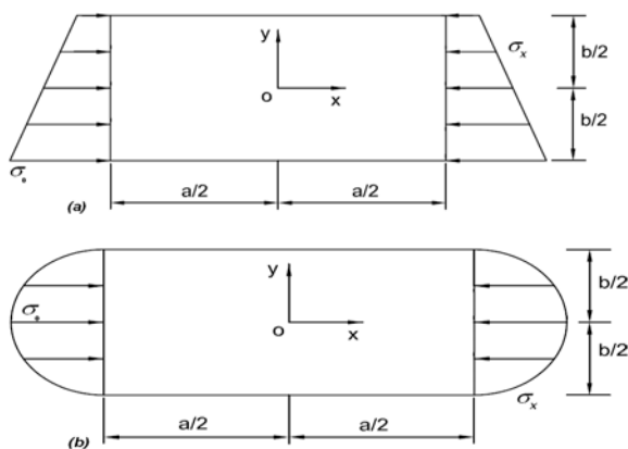
Fig. 2 Rectangular plate under uniaxial edge compressions.
