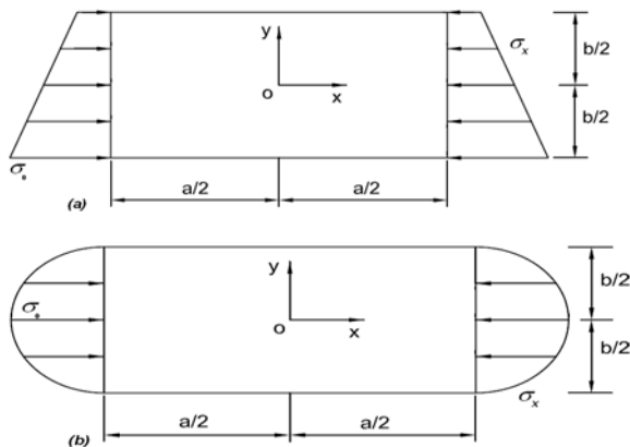
Fig. 2 Rectangular plate under uniaxial edge compressions.
