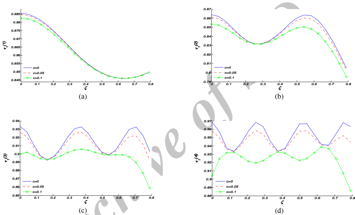
Fig. 8 First four frequency of simply supported stepped beam with a concentrated mass having rotary inertia.
