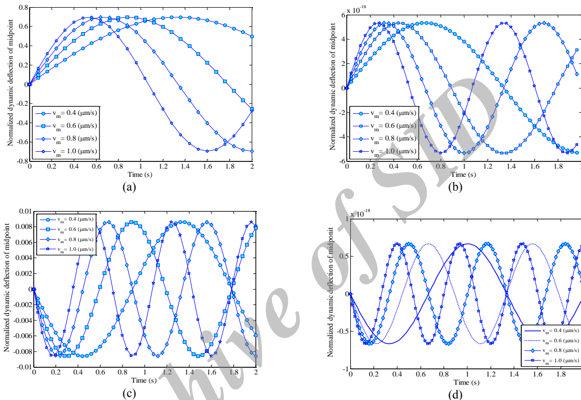
Fig.3 Time history of normalized deflection of MT midpoint for a) 1 st mode b) 2 nd mode c) 3 rd mode d) 4 th mode.
