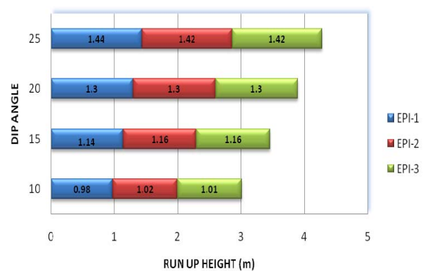
Figure 8. Comparison of dip variation in Dwarka
