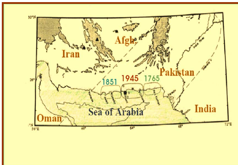
Figure 2. Major earthquakes in MSZ
