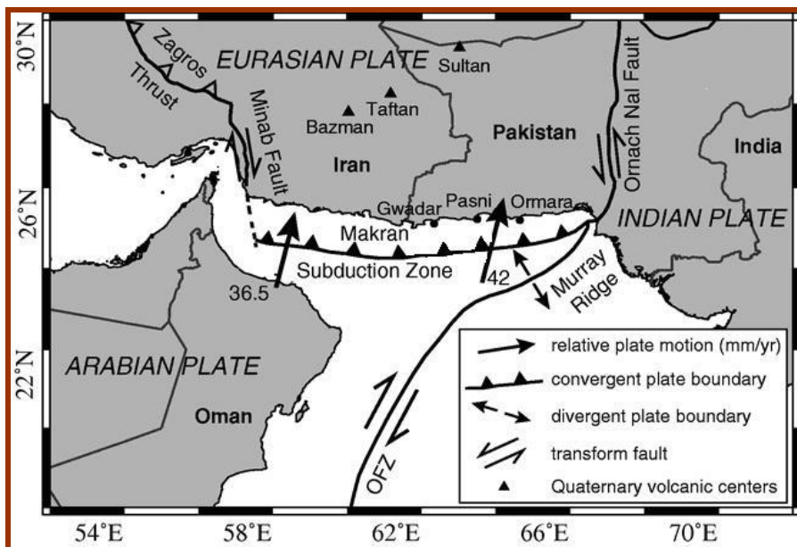
Figure 1. Makran subduction zone (MSZ)
