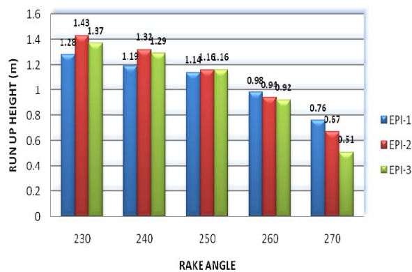
Figure 7. Comparison of rake variation in Dwarka
