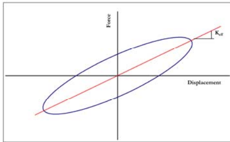
Figure 1. Viscoelastic damper (Trevor & Kelly, 2001)
