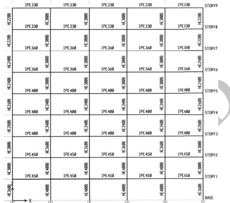
Figure 4. Sample frame without added viscoelastic damper
