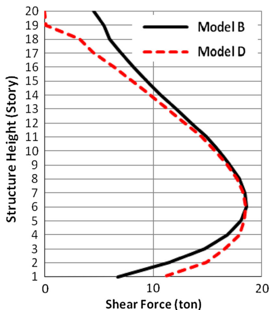
Fig. 23 Link beam shear forces generated by warping
