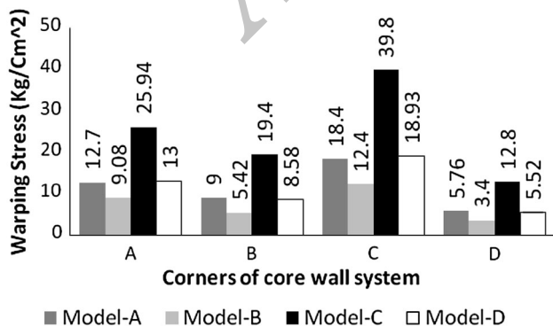
Fig. 15 Comparison of core warping stresses at four positions of core in 17th story level
