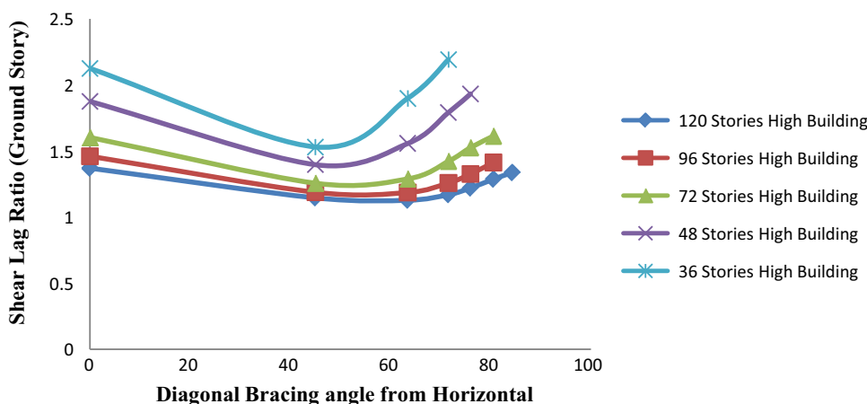
Fig. 16 Variation of shear lag with varying angle of bracing system for buildings of model 3
