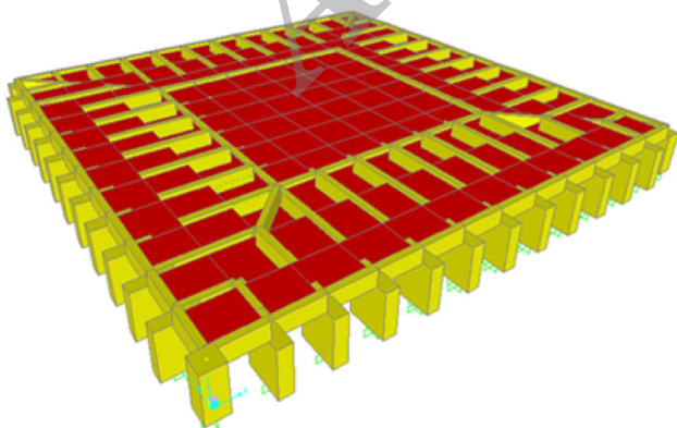
Fig. 4 Perspective view of the ground story
