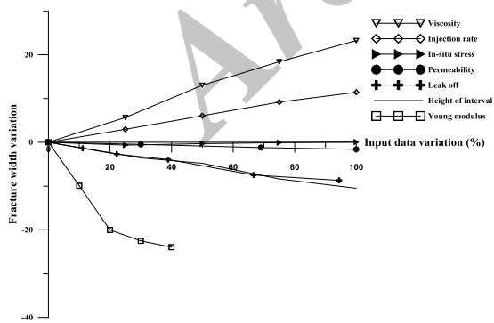
Figure 7. Effect of various parameters on the fracture width
