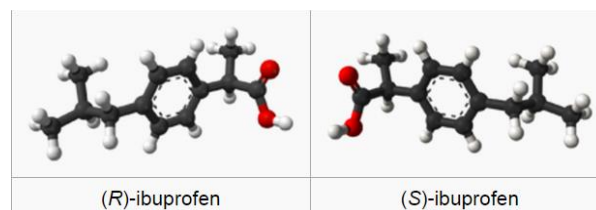
Figure 4. Ibuprofen enantiomers [21]
