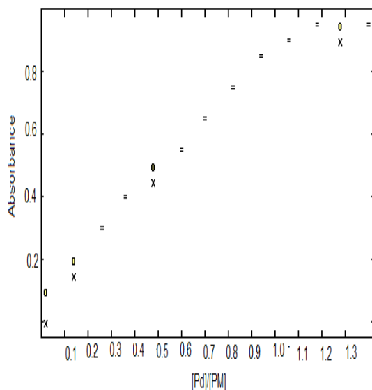
Fig. 6. Computer fits of the plots of absorbance vs. [Pd]/[PM] mole ratios at 25 °C: (x) experimental point, (o) calculated point, (=) experimental and calculated points are the same within the resolution of the plots.
