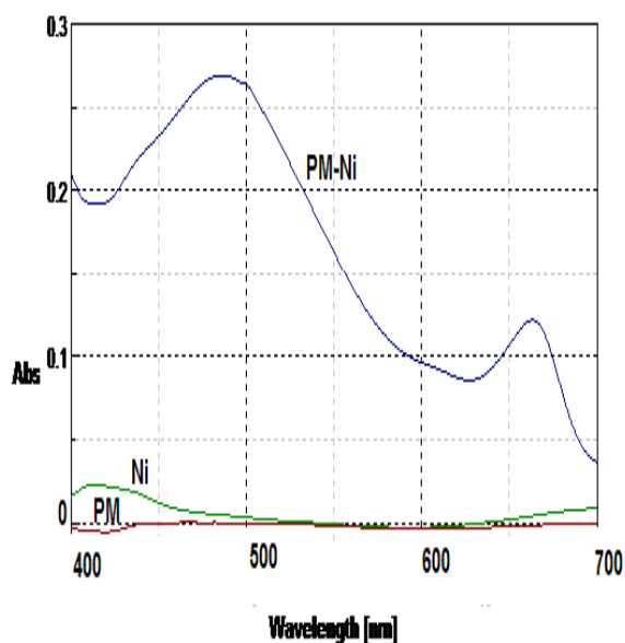
Fig. 5. Absorption spectra of nickel(II) chloride hexahydrate, complex of PM and Ni(II) in the range of 400-700 nm
