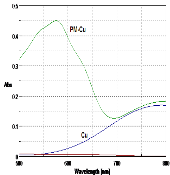
Fig. 4. Absorption spectra of Copper nitrate, complex of PM and Cu(II) in the range of 500-800 nm
