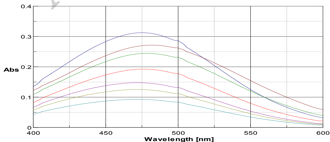
Fig. 3. Absorption spectra of the complex of 0.5-35 \mu\text{g ml}^{-1} PM with Pd (II).
