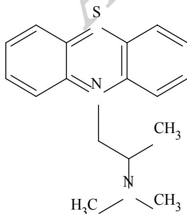
Fig. 1. Structure of promethazine
