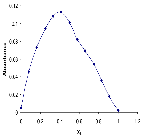
Fig. 2. Continuous variation graph of PM-palladium (II) chloride.
