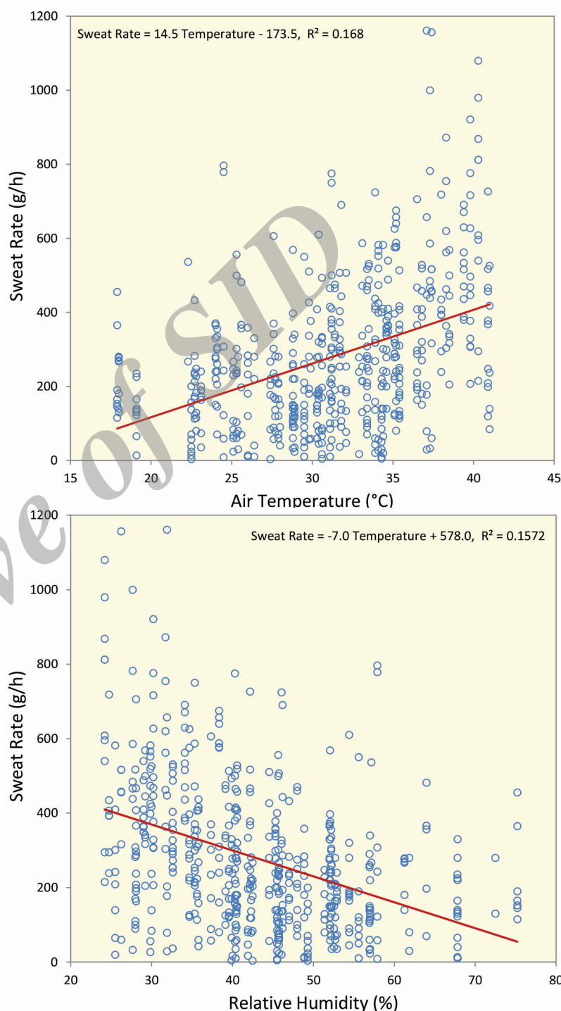
Figure 1: Sweat rate at different temperatures and relative humidity
