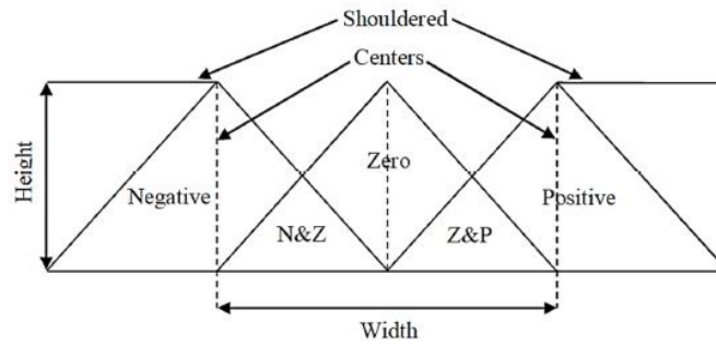
Figure 6- membership functions
