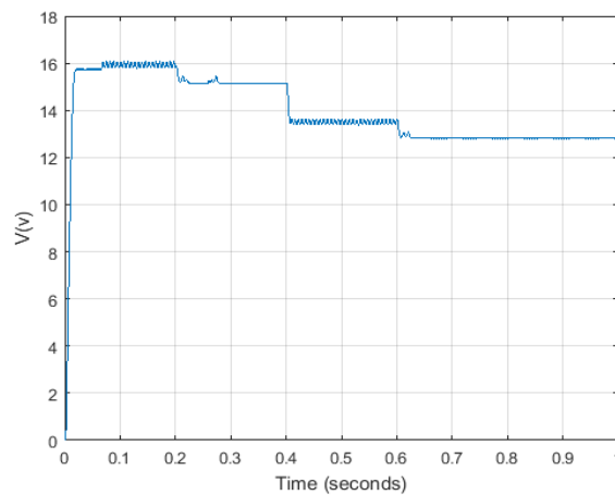
Figure 17-Dual load voltage with fuzzy controller
