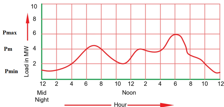
Figure 1: An example of a daily load curve
