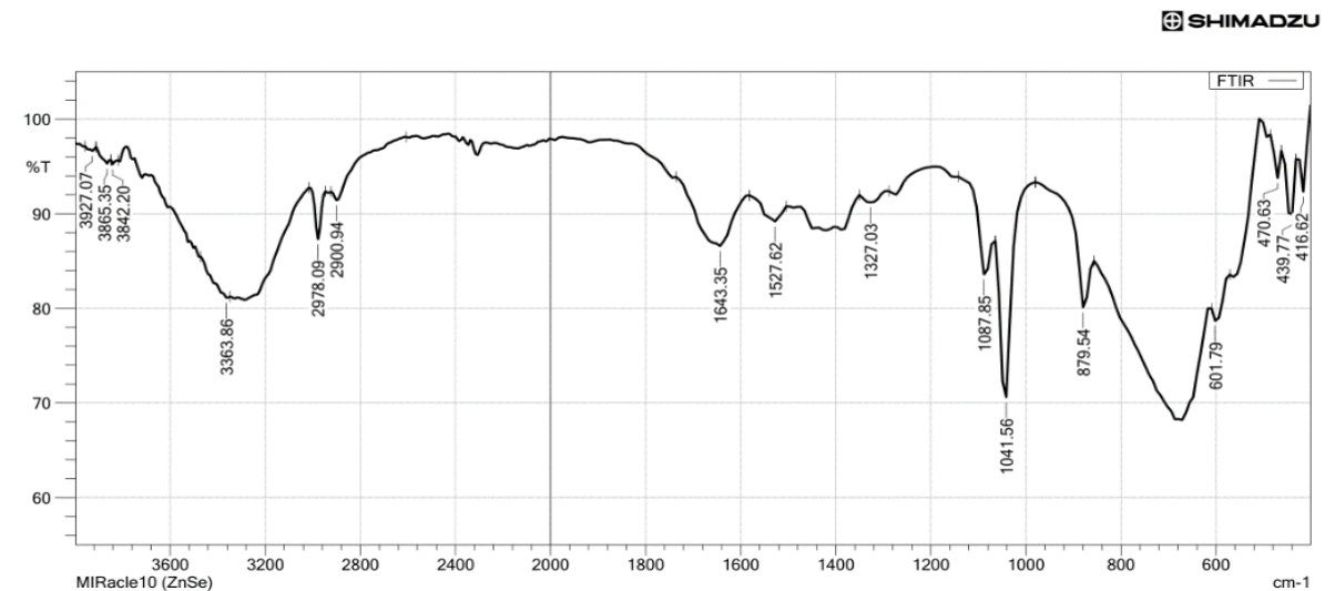
Fig. 3. Papain-CuNPs FT-IR spectrum
