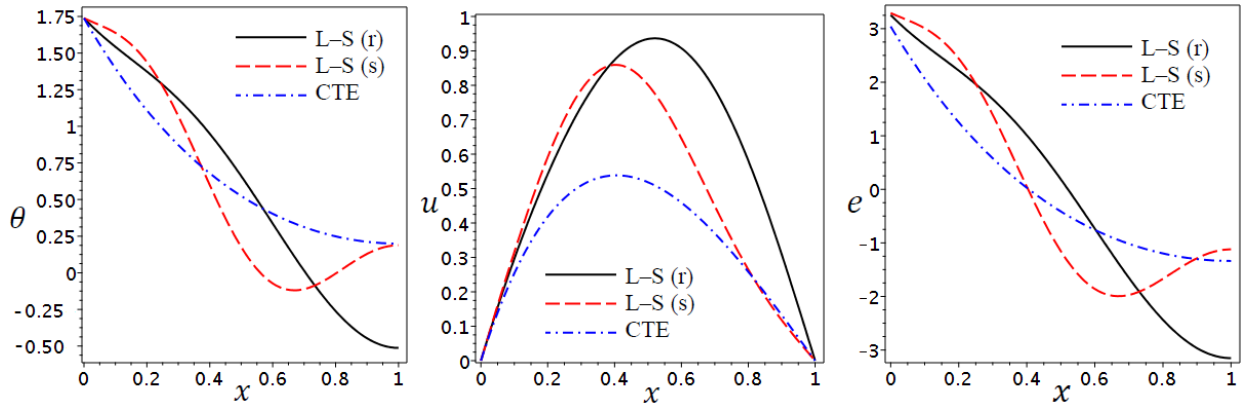
Fig. 3: Distributions of temperature \theta , displacement u , and dilatation e during the skin tissue with fraction parameter \nu = 0.8 .
