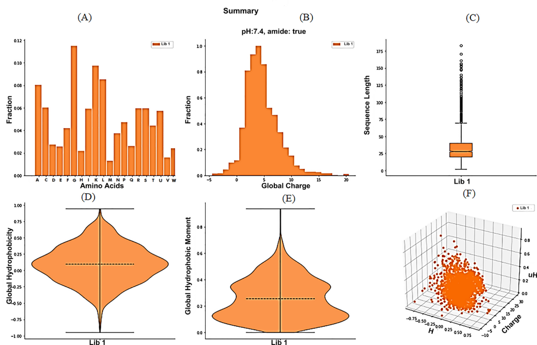
Fig. 2. Global analysis of physicochemical parameters of AMPs global dataset plotted using modiAMP. The global summary plot showing the distribution of basic physicochemical parameters of AMPs like the relative abundance of individual amino acids (A), global charge (B), sequence length (C), global hydrophobicity (D), hydrophobic moment (E) and 3D scatter plot (F) that shows the correlation.
