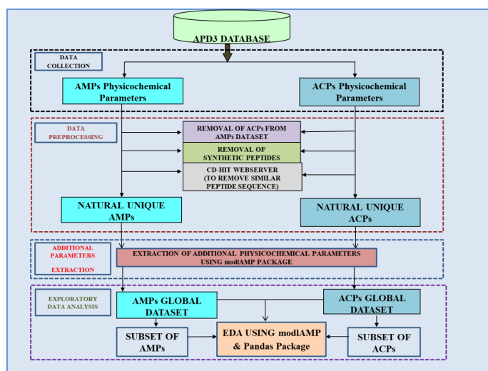
Fig. 1. Overall methodology used for exploratory data analysis of physicochemical parameters of natural AMPs and ACPs.
