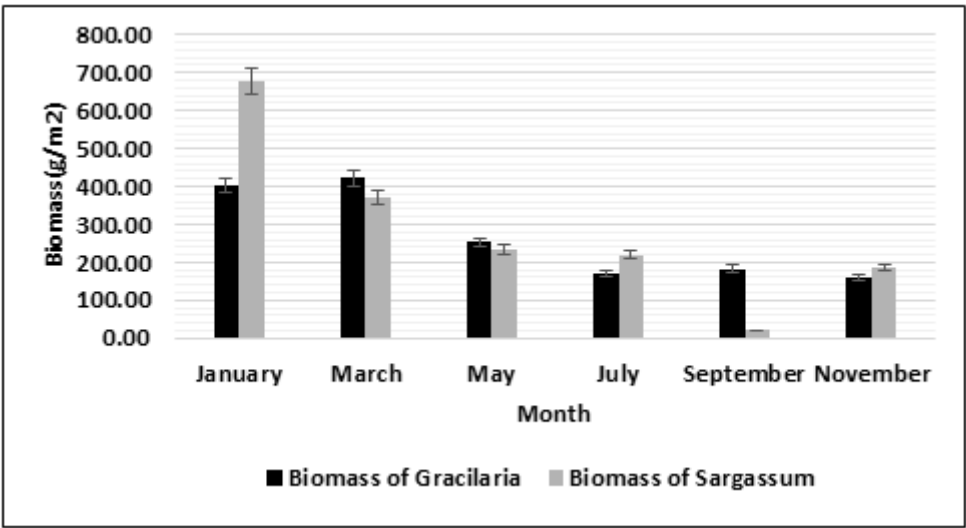
Figure 2: Comparison of average biomass of Gracilaria and Sargassum (g/m²). Error bars show standard error.
