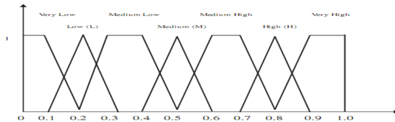
Fig. 2: Chen and Huang’s scale to convert linguistic terms to fuzzy numbers
