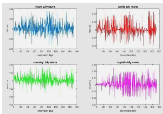
Fig. 1: Daily return of assets in this study
