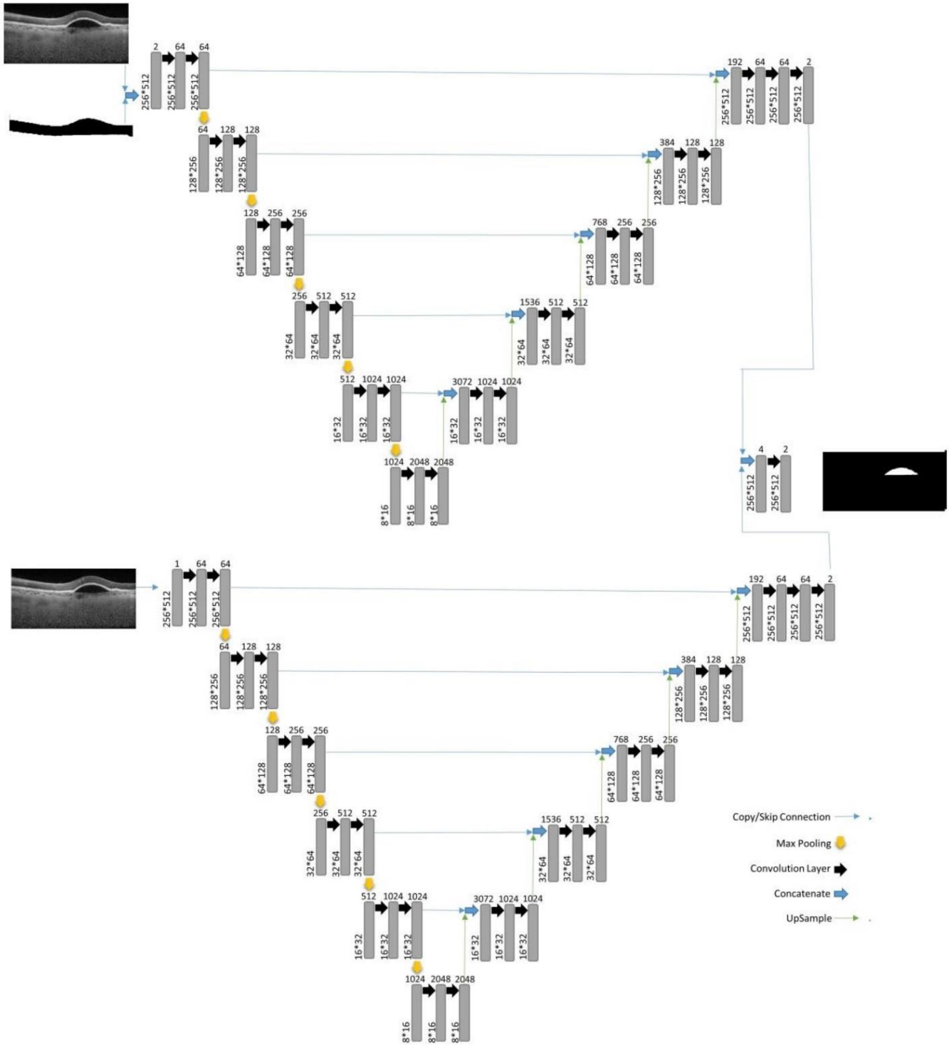
Fig. 4. Proposed TPFCN for fluid segmentation.
