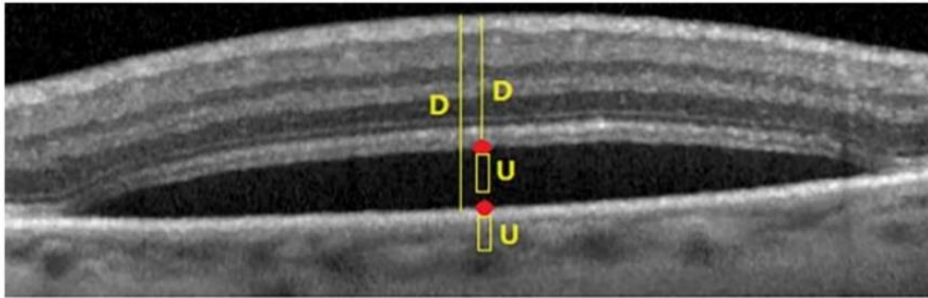
Fig. 2. Illustration of U and D.
