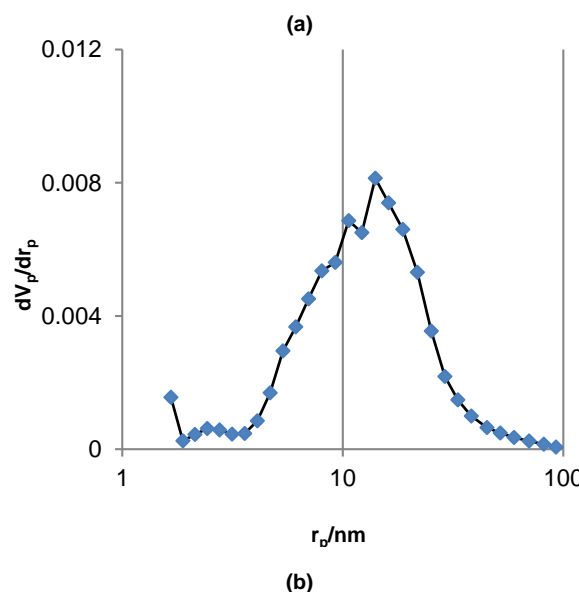
Fig. 4. (a) Nitrogen adsorption/desorption isotherm, (b) Pore size distribution of Fe 3 O 4 /Date Kernels adsorbent.
