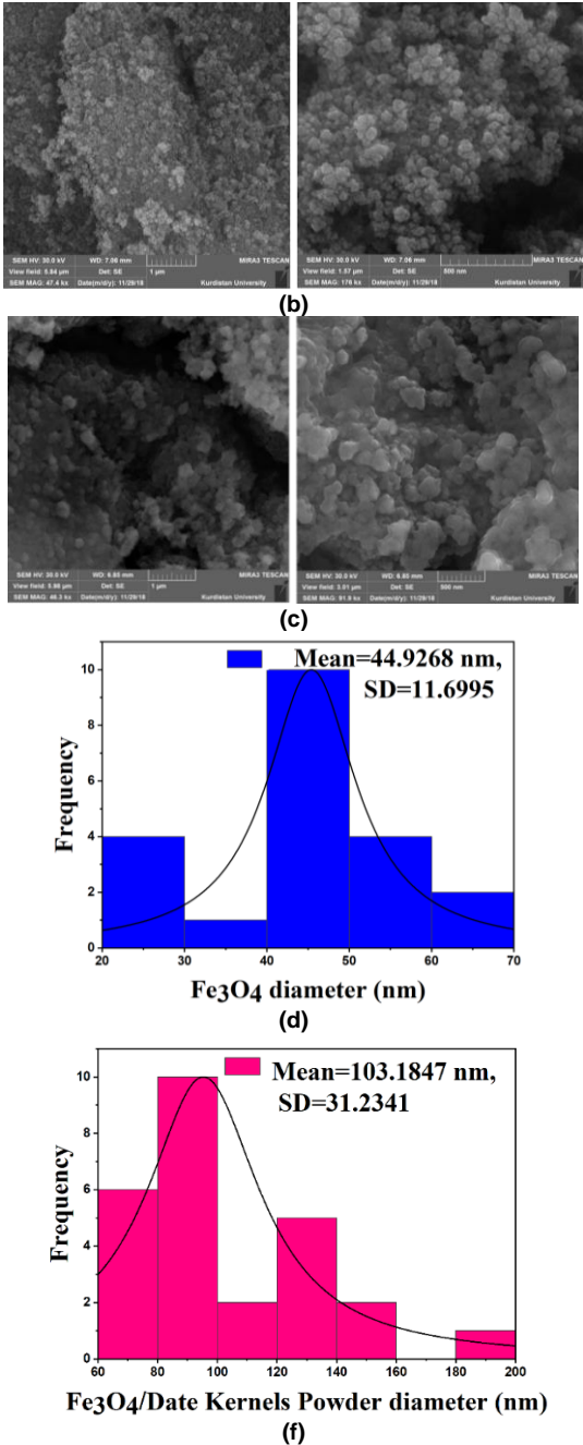
Fig. 2. Morphology and histogram of size of adsorbents, (a) DKP, (b) Fe 3 O 4 , (c) Fe 3 O 4 /DKP, Histogram of size of d) Fe 3 O 4 , and f) Fe 3 O 4 /DKP.
