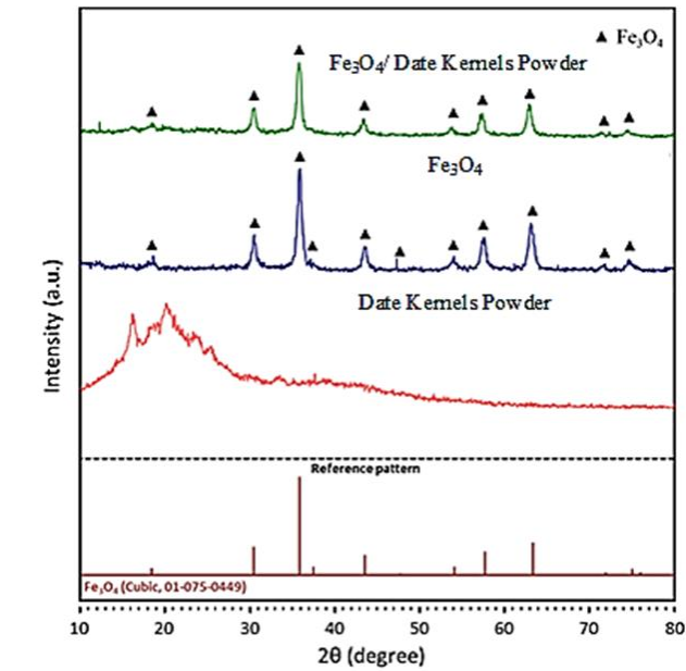
Fig. 1. XRD of DKP, Fe 3 O 4 and Fe 3 O 4 /DKP.
