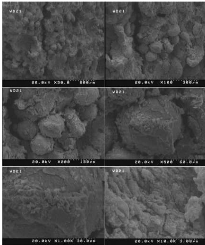
Fig. 11. SEM images of the sample containing dune sand at different magnifications
