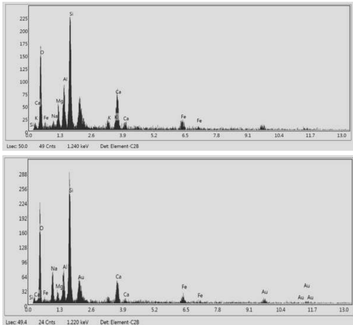
Fig. 13. EDAX examination of the CBW powder (top) and CBW-based geopolymer sample (made with 8M NaOH solution and WG/NaOH=2)
