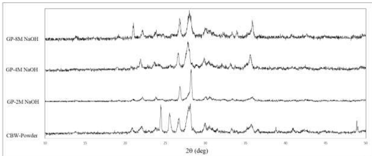
Fig. 12. XRD examination of the CBW powder and CBW-based geopolymer sample (made with 2, 4 and 8M NaOH solution, and WG/NaOH=2)
