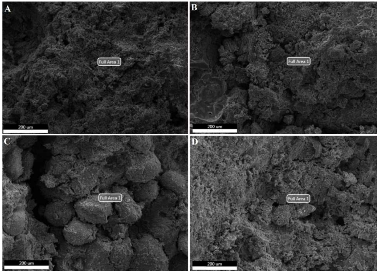
Fig. 10. SEM images of CBW powder-based geopolymer samples without filler (A), with CBW fillers (B), the dune sand filler (C), and the washed sand filler (D)
