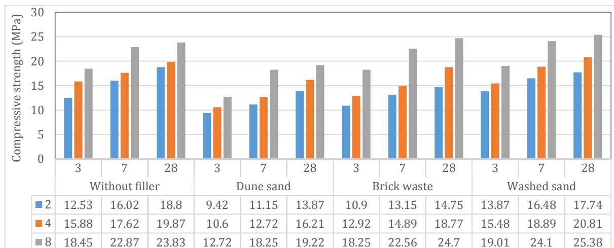
Fig. 8. Compressive strength of geopolymer bricks with WG/NaOH=2
