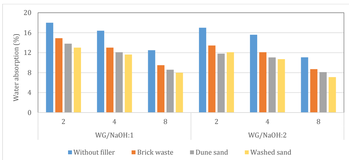
Fig. 9. The 28-day water absorption of brick-shaped geopolymer samples
