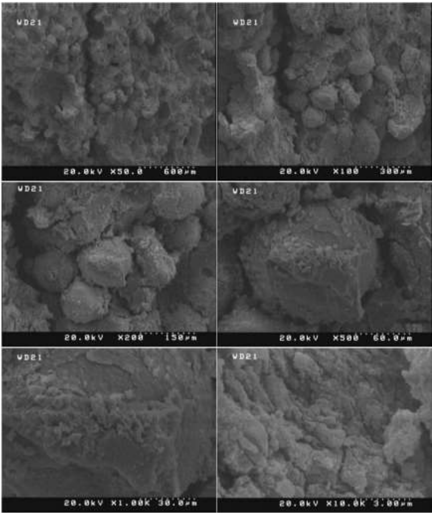
Fig. 11. SEM images of the sample containing dune sand at different magnifications
