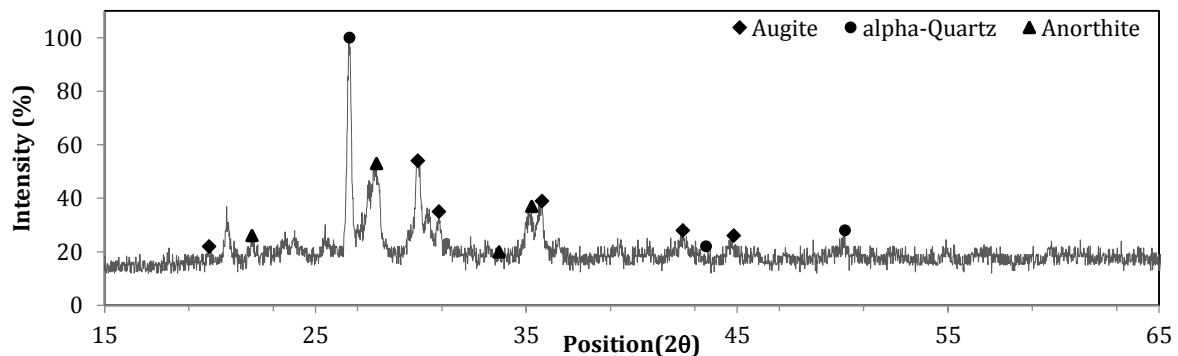
Fig. 4. XRD examination of CBW powder
