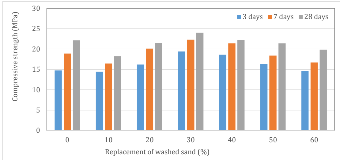
Fig. 6. Compressive strength of cubic geopolymer samples made with different percentages of washed-sand
