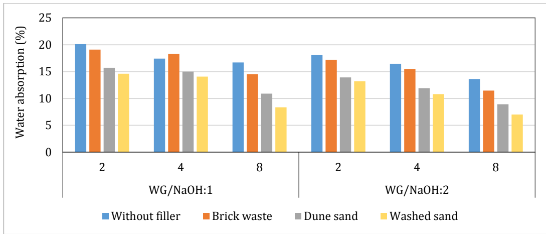
Fig. 7. Water absorption of 28-day cubic geopolymer samples (in the samples made with the filler, 50% filler replacement with the CBW powder was used).
