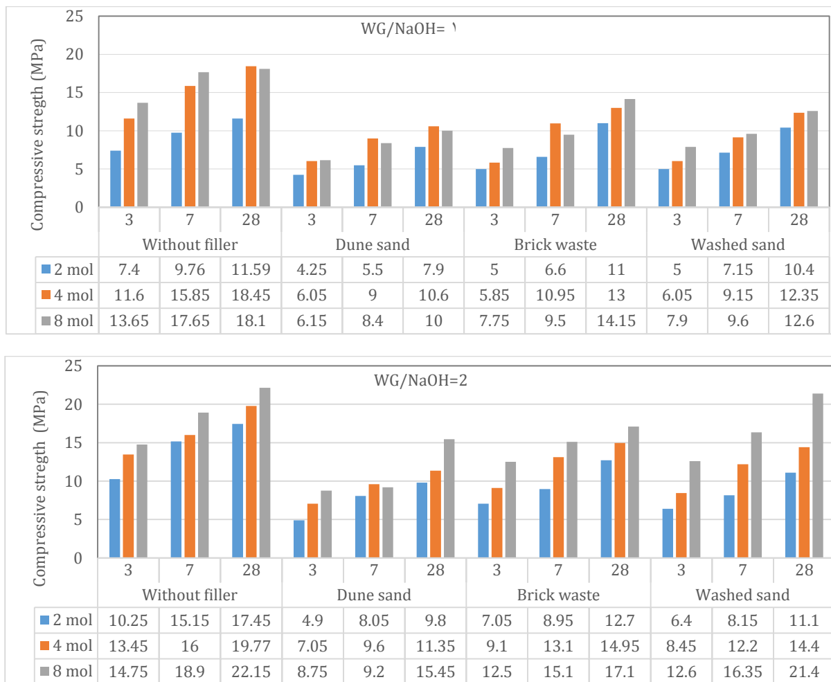
Fig. 5. Compressive strength of 3-, 7- and 28-day cubic geopolymer samples made without using a filler or with different fillers including dune sand, brick waste and washed sand
