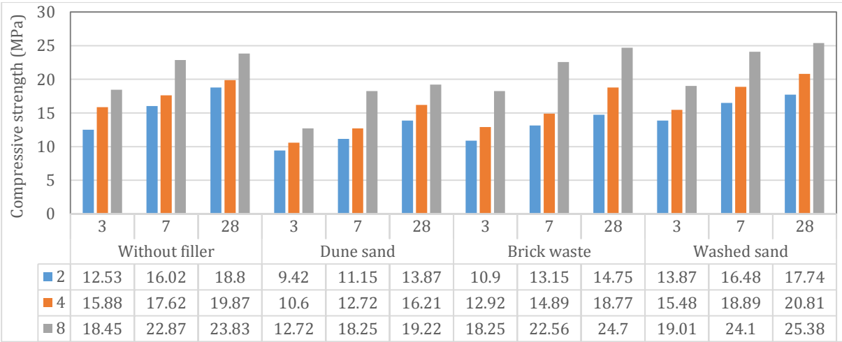
Fig. 8. Compressive strength of geopolymer bricks with WG/NaOH=2
