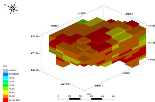
Figure7. Estimated block model
