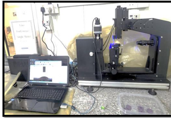
Figure 1: Contact angle goniometer with a high digital video camera and a monitor
