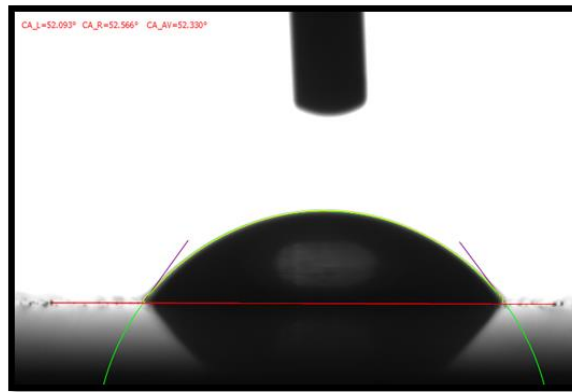
Figure 2: Contact angle measurement on both sides of the drop by software
