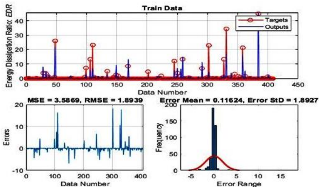
Figure 15- The output results of the GMDH model in the MATLAB environment during the training phase in Hasan Abad station
