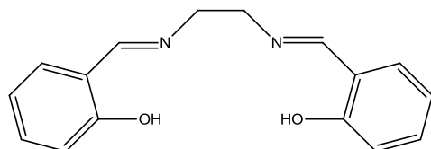
FIGURE 1 The chemical structure of traditional Salen ligand
