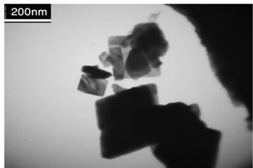
Figure 2. TEM image of AC-TW
