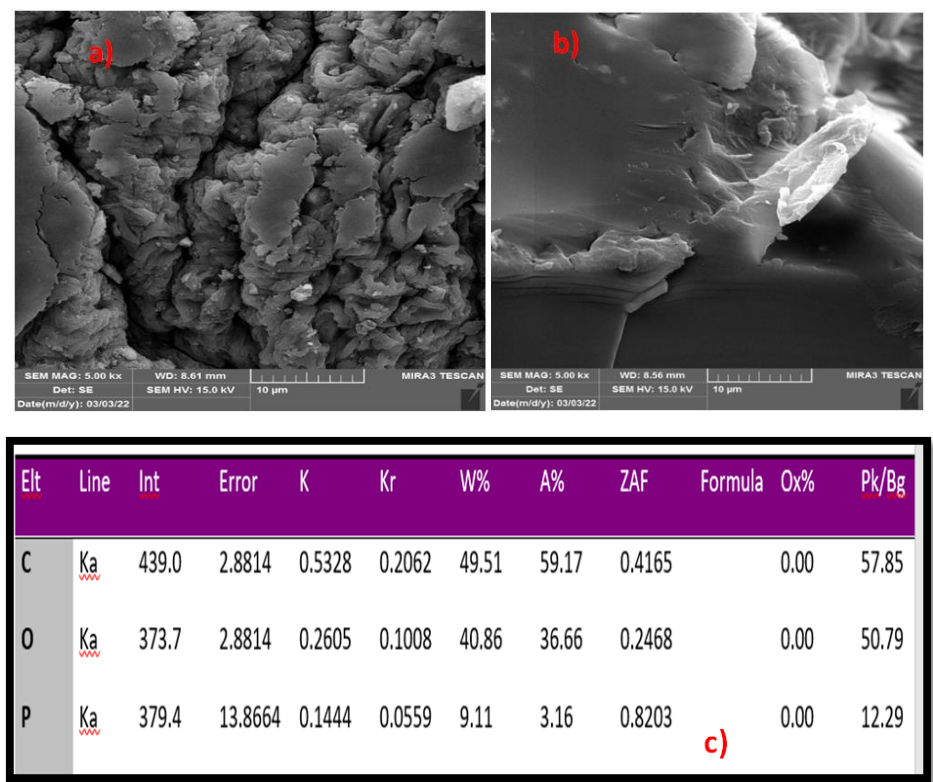
Figure 1. The scanning electron microscope (SEM) technique (a) before adsorption, (b) after adsorption, and (c) EDX of AC-TW
