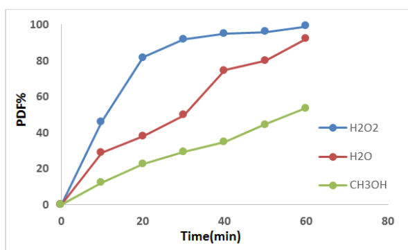
Figure 7. Effect \text{H}_2\text{O}_2 on photocatalytic. Experimental conditions: 0.3 g, TC drug concentration 50 mg/L, and light intensity 1.2 mW/cm 2 .
