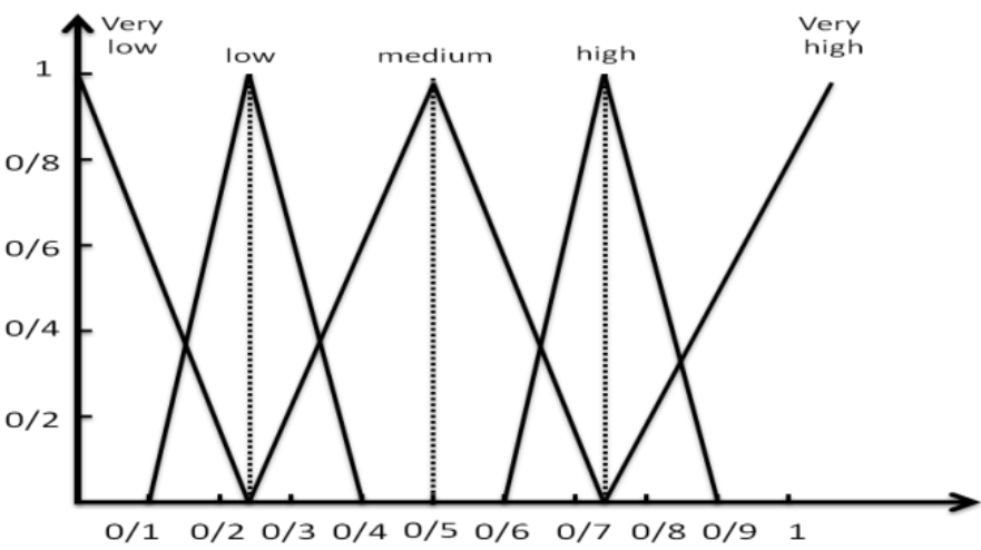
Fig. 1: Triangular fuzzy number of verbal variables
