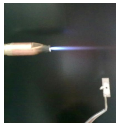
Figure 1. Soldering phase
