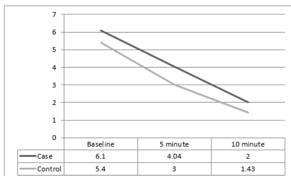
Figure 1: Comparing the trend of pain reduction 5 ( p = 0.88 ) and 10 ( p = 0.72 ) minutes after lidocaine injection between case and control groups.
