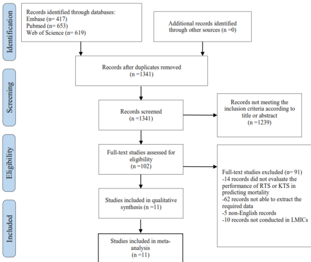
Figure 1: Flow diagram of systematic search for the meta-analysis considering the ability of the Revised Trauma Score and Kampala Trauma Score in predicting mortality. RTS, Revised Trauma Score; KTS, Kampala Trauma Score; LMICs, Low and Middle-Income Countries.
