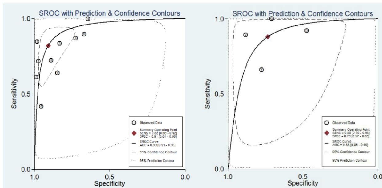
Figure 3: Summary receiver operating characteristic curves (SROC) of Revised Trauma Score (left) and Kampala Trauma Score (right). AUC, area under the receiver operating characteristic curve.
