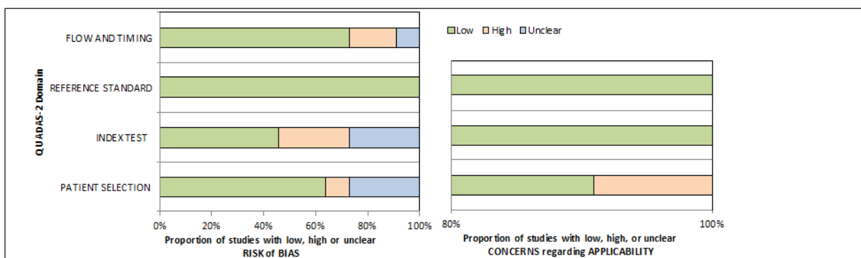
Figure 2: Quality assessment of included studies using QUADAS-2.
