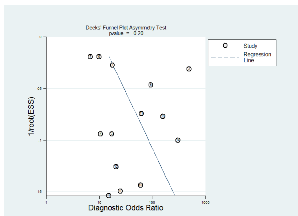
Figure 4: The funnel plot for assessment of publication bias.
