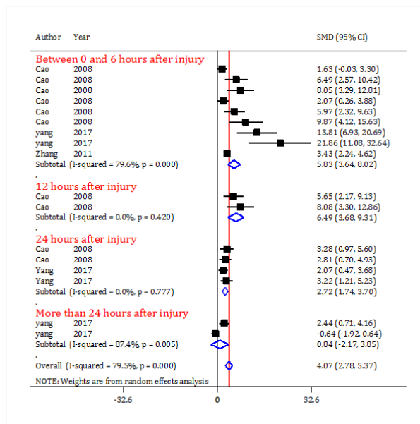
Figure 4: Forest plot of CSF S-100β in spinal cord injury. Animal studies showed that the mean level of CSF S-100β is higher in animals with spinal cord injury during the first 24 hours after trauma. CI: Confidence interval; SMD: Standardized mean difference.
