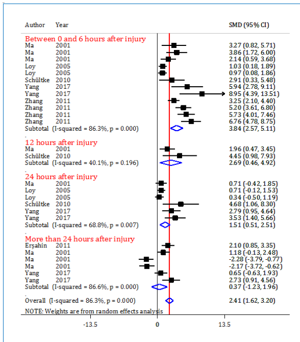
Figure 3: Forest plot of serum S-100β in spinal cord injury. Animal studies showed that the mean level of serum S-100β is higher in animals with spinal cord injury during the first 24 hours after trauma. CI: Confidence interval; SMD: Standardized mean difference.
