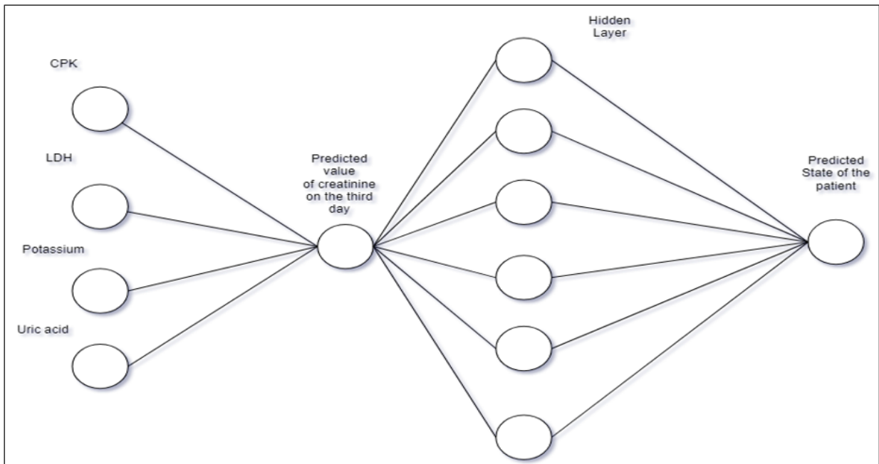
Figure 1: The architecture of the first model from available data (FC_NN). CPK: Creatine phosphokinase; LDH: lactate dehydrogenase.
