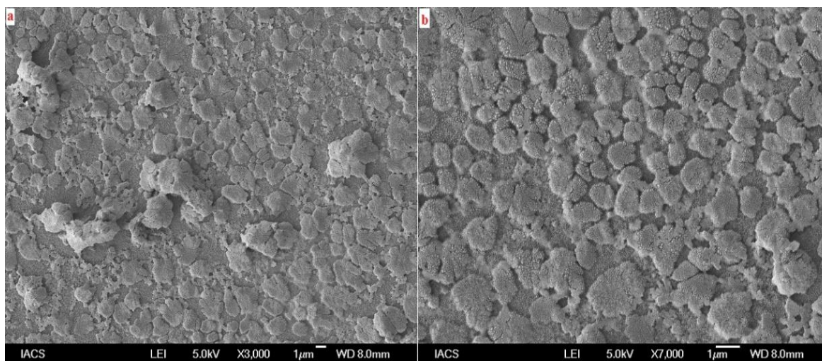
Figure3. Field emission scanning electron microscope images of green synthesized gold nanoparticles.
