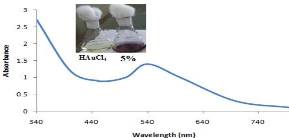
Figure 1. UV-vis-absorption spectra of 5% methanol extract phytochemically synthesized gold nanoparticles. The inset image shows the 1mM HAuCl 4 solution and green synthesized gold nanoparticles solution.
