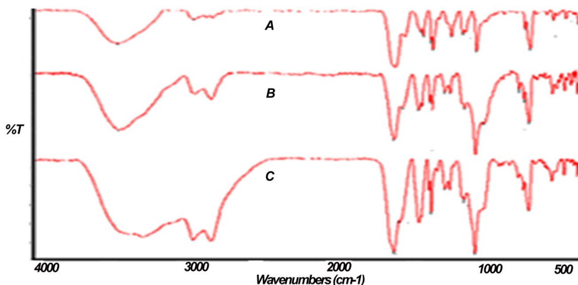
Figure 2. FTIR spectra of three SWNT-PEIs: A) V1.8 B) V10 C) V25.
