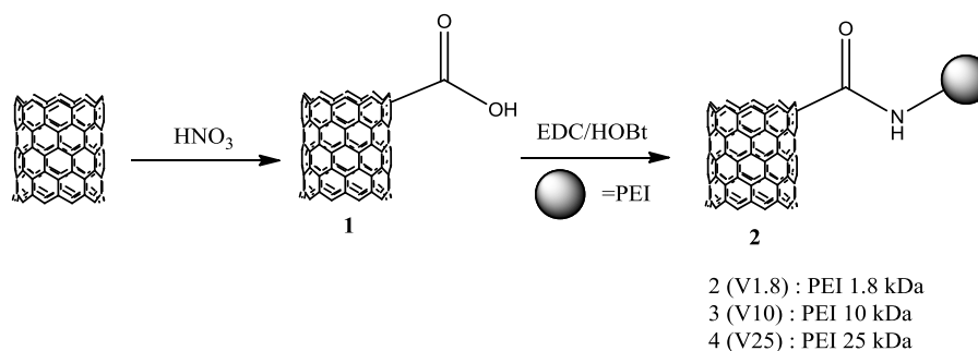
Figure 1. Schematic presentation of synthetic steps used in preparation of SWNT-PEIs conjugates.
