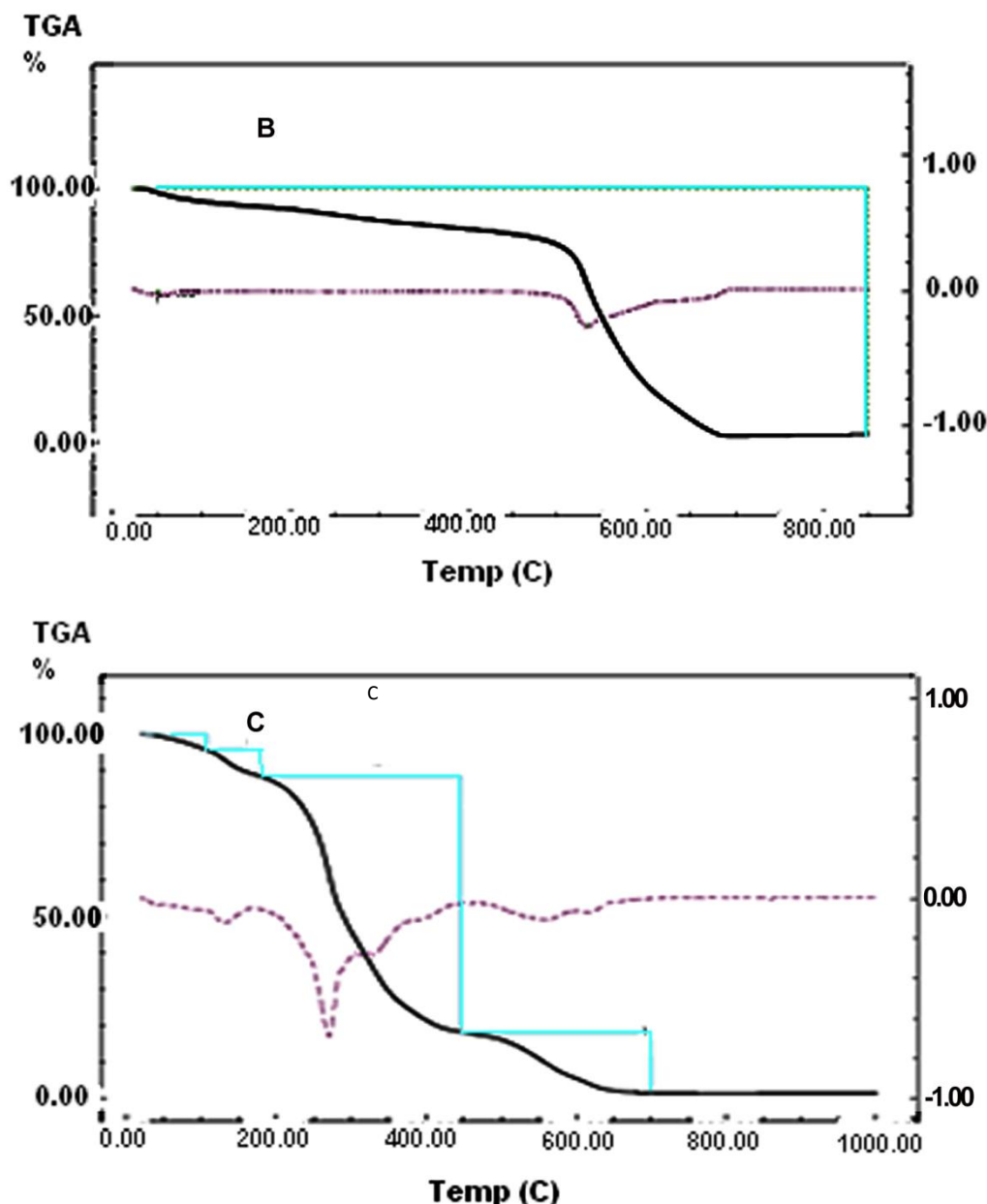
Figure 4. TGA diagrams of A) pristine SWNT B) SWNT-COOH C) SWNT-amide-PEI1.8 (V1.8).
