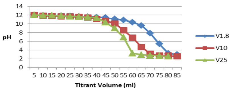
Figure 5. Buffering capacity of vectors was measured by titration with HCl 0.1 N solution.
