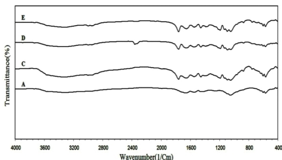
Fig. 3. FTIR spectrum of hydroxyapatite, sample A and samples C-E
