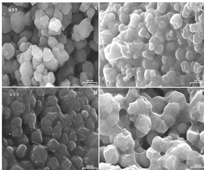
Fig. 4. FESEM image of the (A) hydroxyapatite nanoparticles, (B) Sample A , (C) sample B, (D) sample E
