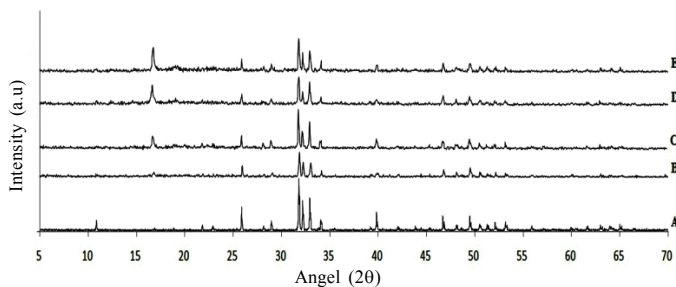
Fig. 2. XRD curves of samples A-E
