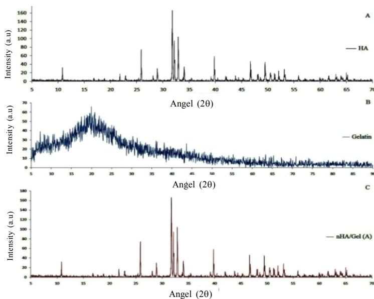
Fig. 1. XRD curves for (A) pure hydroxyapatite nanoparticles, (B) pure gelatin, (C) nHA /Gel nanocomposite
