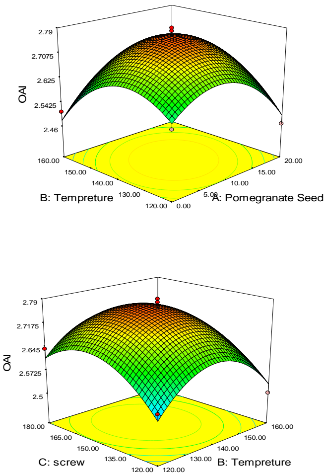
Figure 1. Effects of pomegranate seed powder, screw speed and extruder temperature on OAI
