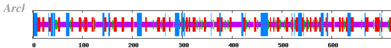
Fig. 1. Graphical representation of SOPMA results. Red, Extended strand; blue, Alpha-helix; green, Beta turn, and yellow, Random coil
