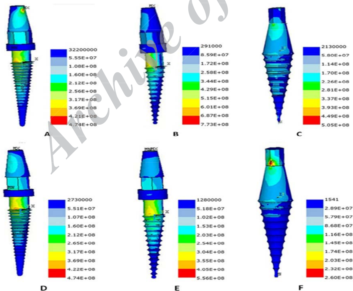
Figure 2: VonMises stress distribution within three MDIs under static loading. A to C, D3 bone; D to F, D2 bone; (A, D) Dentis; (B,E) Dio; (C,F) Osteocare.
