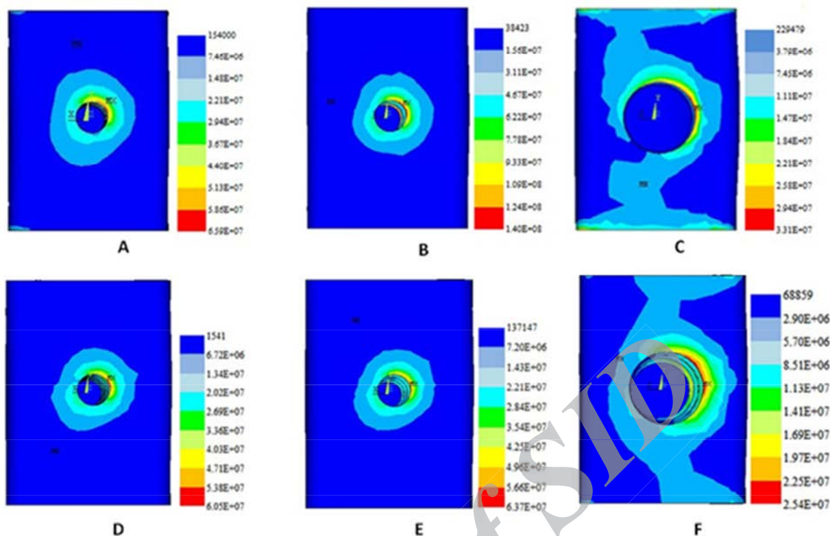
Figure 3: VonMises stress distribution within cortical bone under static loading. A to C, D3 bone; D to F, D2 bone; (A,D) Dentis; (B,E) Dio; (C,F) Osteocare.
