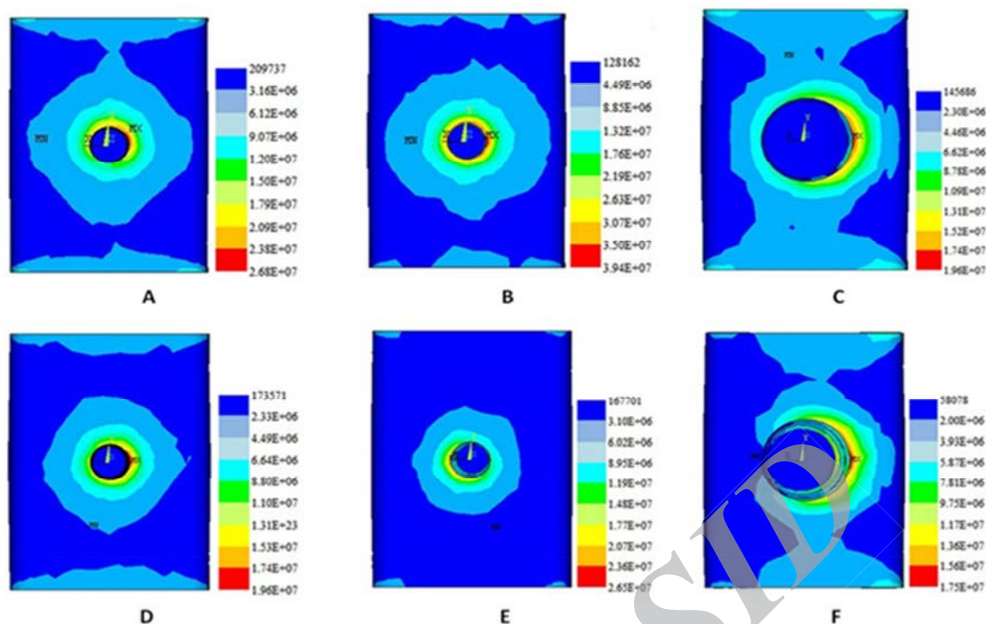
Figure 5: VonMises stress distribution within cortical bone under dynamic loading. A to C, D3 bone; D to F, D2 bone; (A,D) Dentis; (B,E) Dio; (C,F) Osteocare.
